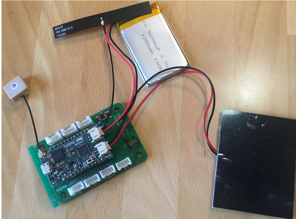
Fig. 36: The SODAQ ONE-EU-RN2483-V3 installed on a ONE Base board with attached GPS antenna (left), LoRa patch antenna (top), a 1200 mAh lithium polymer (LiPo) battery (top), and an attached 0.5W photovoltaic panel.
